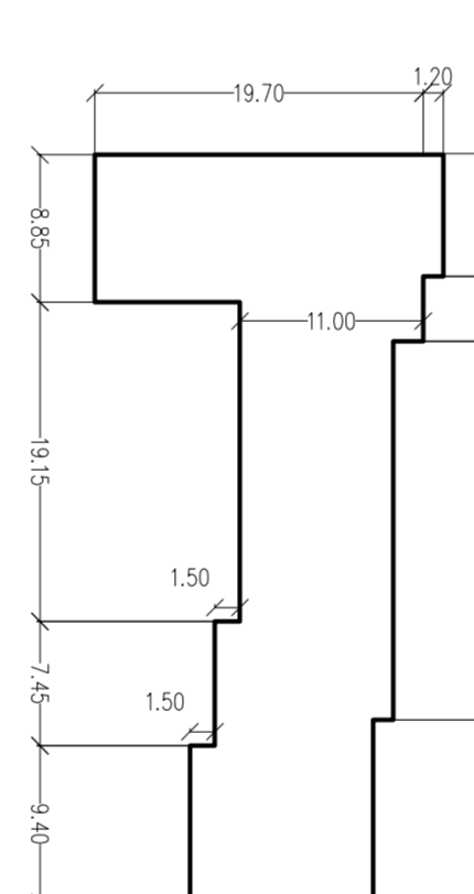
PIANTA A QUOTA +3,40, 6,45, 9,50, 12,55, 15,60, 18,65
